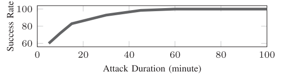
Fig. 5. Impact of attack duration on the success rate of weight determination.
