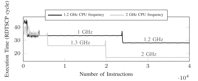
Fig. 3. Illustration of AMX frequency adjustment.
