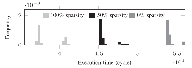
Fig. 2. Execution time with varying operand sparsity.
